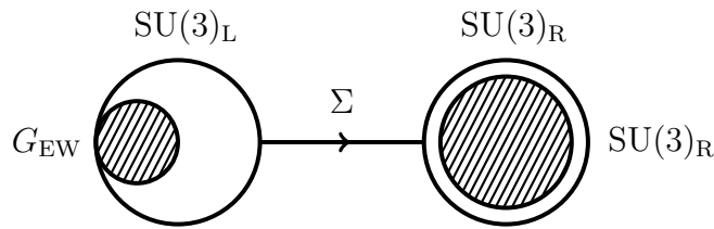
Figure 14: Full symmetry structure of the minimal moose little Higgs model. Shaded blobs represent gauged subgroups. We explicitly show that only the ‘diagonal’ subgroups are gauged.
