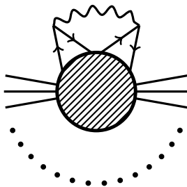
Figure 9: ‘Cat diagram’ adapted from [151]. Despite the silly appearance, the key point is that the photon couples to the electric current J_\mu = e\bar{\Psi}\gamma_\mu\Psi (‘ears’) formed from interactions with fundamental quarks in the strongly coupled sector. The ‘whiskers’ are the pseudo-Goldstone external states when expanding the U(x) field in (4.28). The contribution to the charged meson masses come from the ‘two whisker’ diagram.
