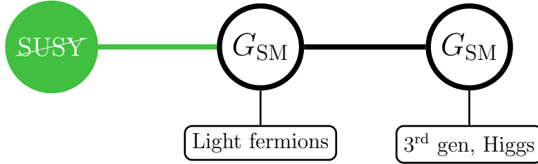
Figure 15: Schematic moose diagram for natural SUSY.
