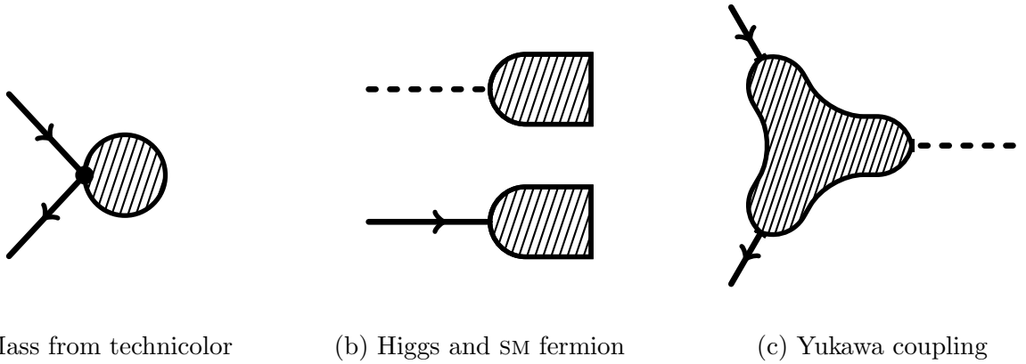
Figure 11: Fermion couplings to the composite sector, represented by shaded blobs. (a): Bilinear coupling of fermions to the composite sector (4.56) lead to fermion masses from the condensate of techniquarks. (b): Partial compositeness scenario. In addition to the Higgs being part of the strong sector, the elementary SM fermions mix linearly with strong sector operators with the same quantum numbers. (c): Yukawa interactions are generated through the strong sector dynamics. Adapted from [160].
